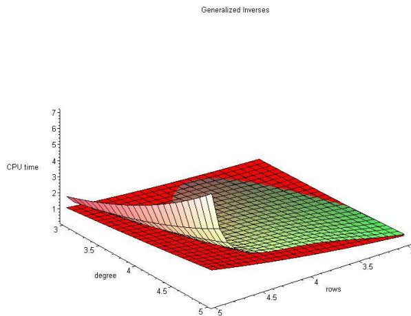
Diagram 1. Graph of the CPU time= F(\text{rows}, \text{degree}) in both algorithms DFTGI and [8].
