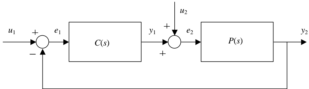
Figure 1: The unity Feedback system S(P, C)
